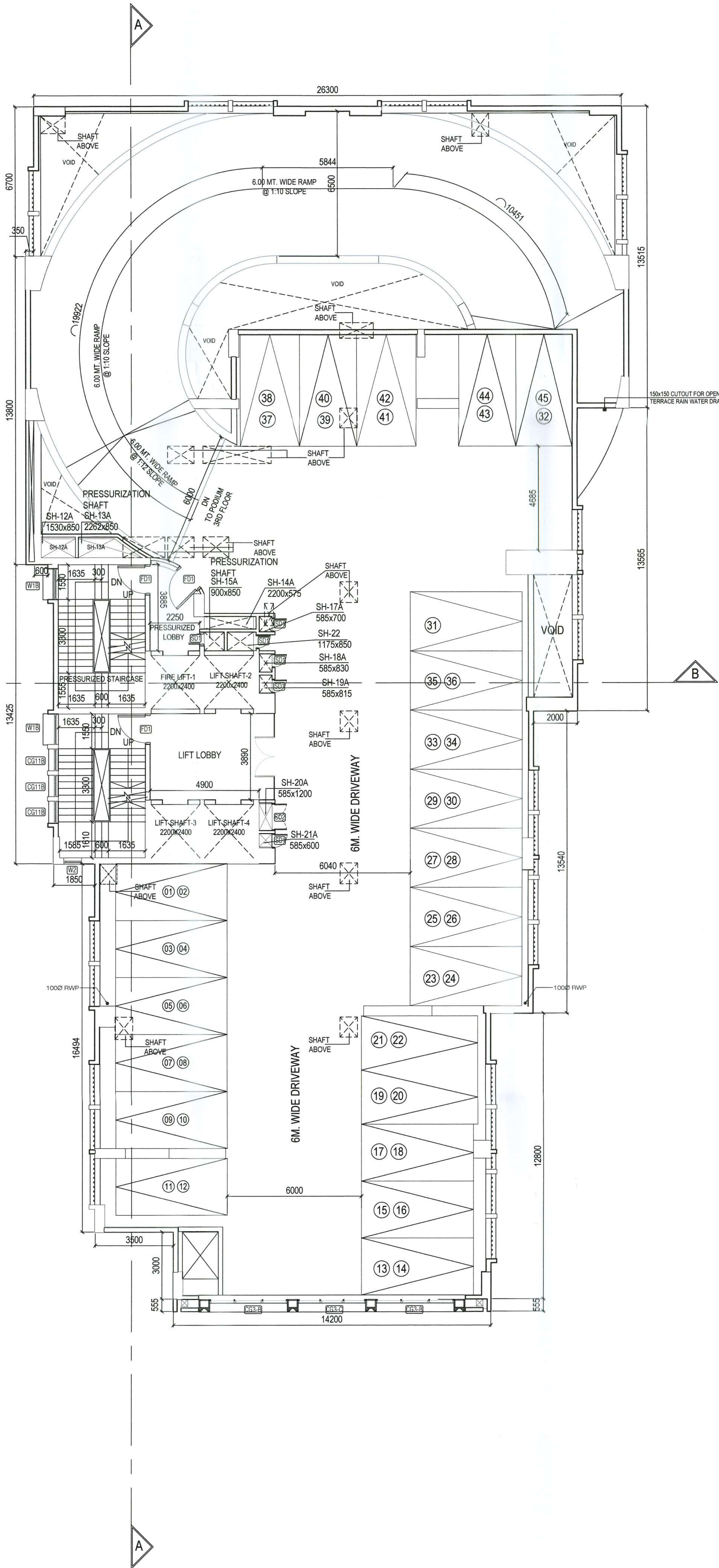
PODIUM - 4TH LEVEL SCALE : 1 : 100
