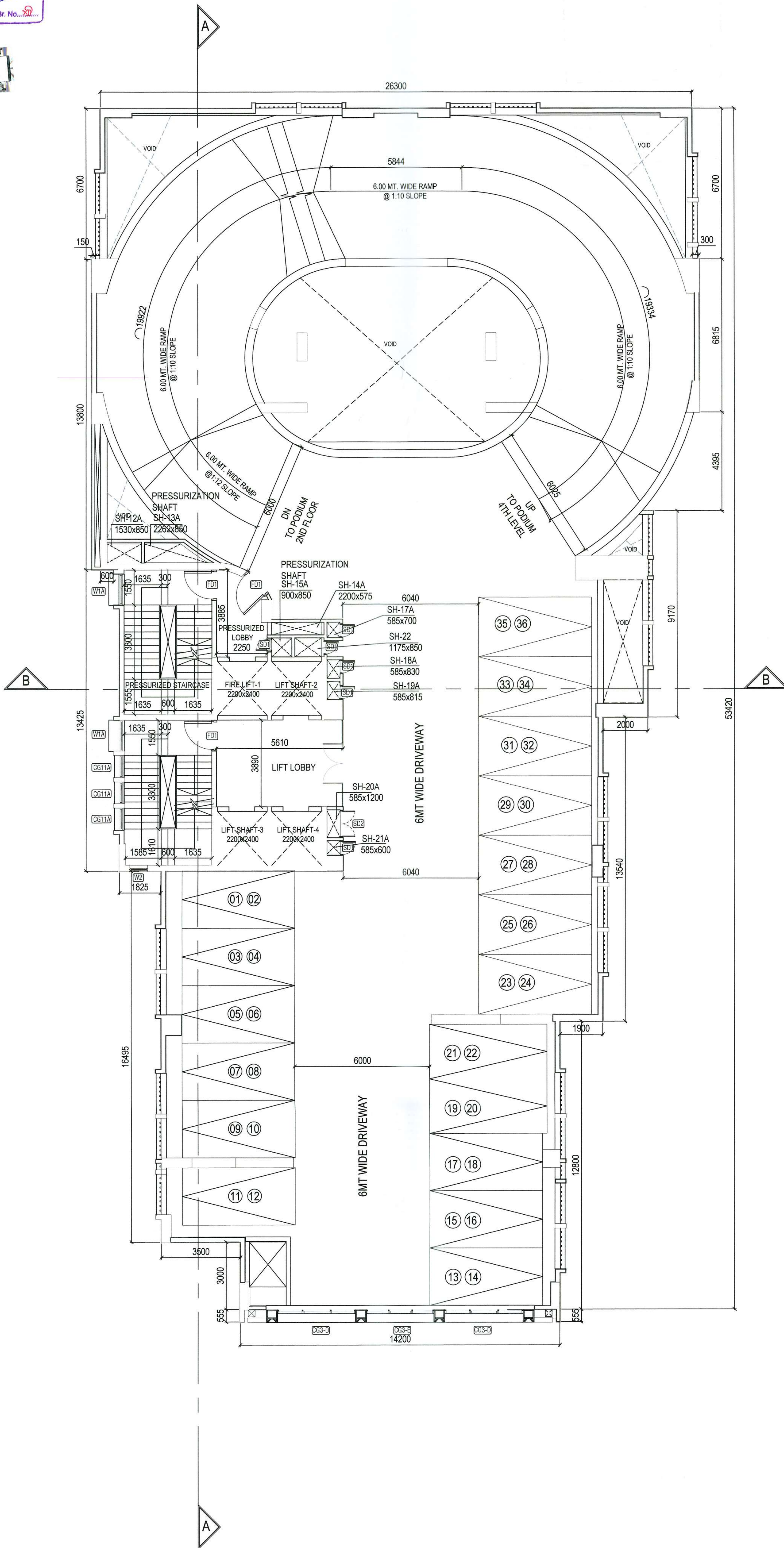
PODIUM - 3RD LEVEL SCALE : 1 : 100
